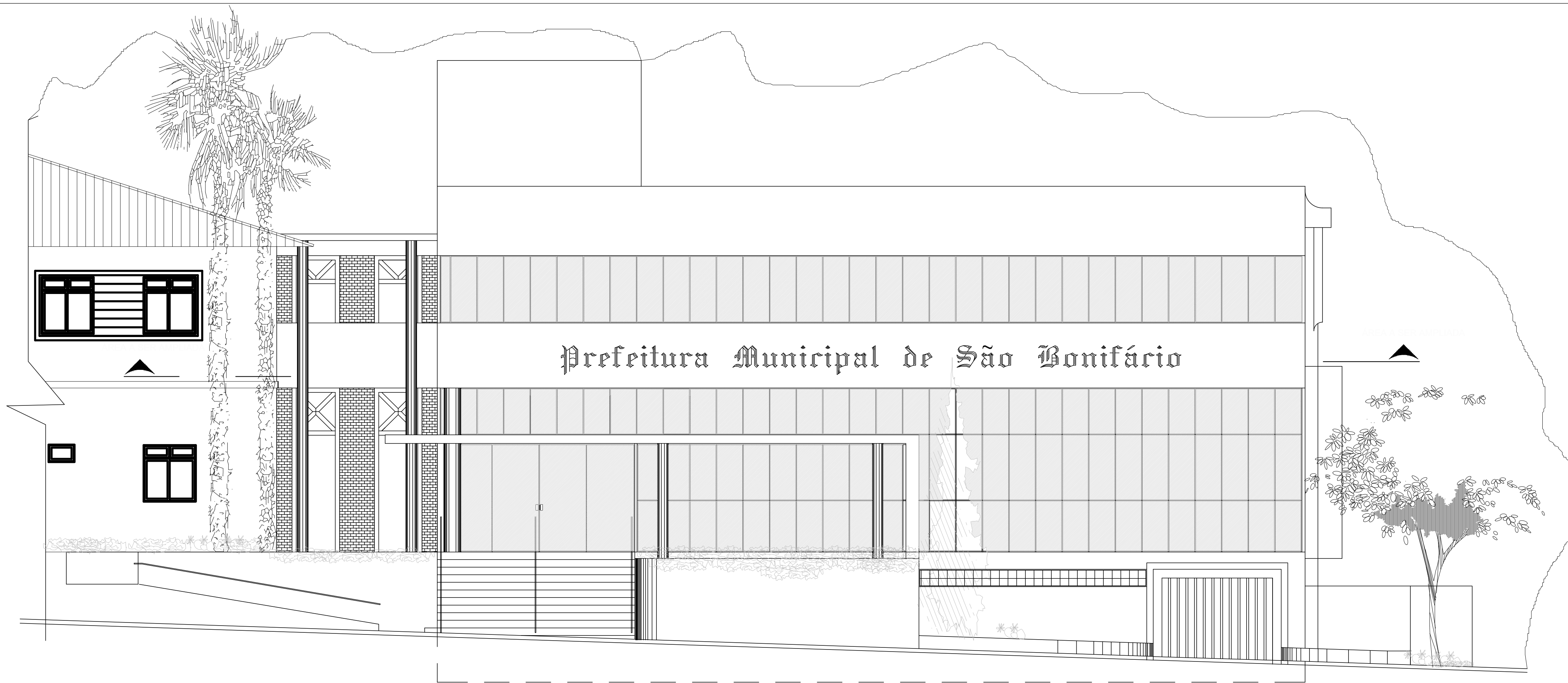
FACHADA PRINCIPAL ESCALA 1:50
